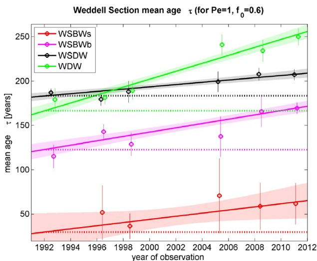
Fig. 23 Time series of ages in WDW, WSDW, and WSBW (left) and C_{\text{ant}} at the Weddell Sea section (location see Fig. 18). The stippled lines show the expected trends in these water masses when assuming a steady state
