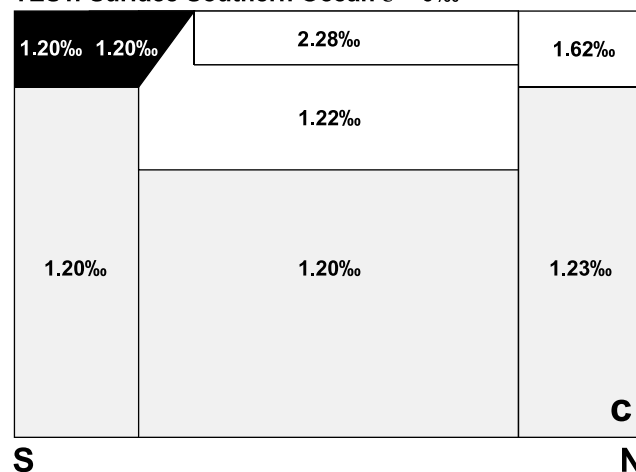
Figure 6. Results of the 8-box model. (a) The model architecture, modified from Toggweiler [1999], with water fluxes in Sv (solid lines) and particulate export (dashed gray arrows). Boxes are p : southern polar surface, s : subantarctic surface, l : low-latitude surface, n : northern high-latitude surface, m thermocline and intermediate, ds : deep southern, dl : deep low-latitude, dn : deep northern box. Model results with isotope fractionation during utilization (represented by the isotope effect \epsilon ) prescribed (b) throughout the surface ocean and (c) everywhere in the surface ocean except the surface Southern Ocean boxes (filled). It can be seen that the North Atlantic–Southern Ocean \delta^{30}\text{Si} gradient produced by the control model in Figure 6b disappears in the test case in Figure 6c. Modeled Si concentrations are identical for both model runs.
